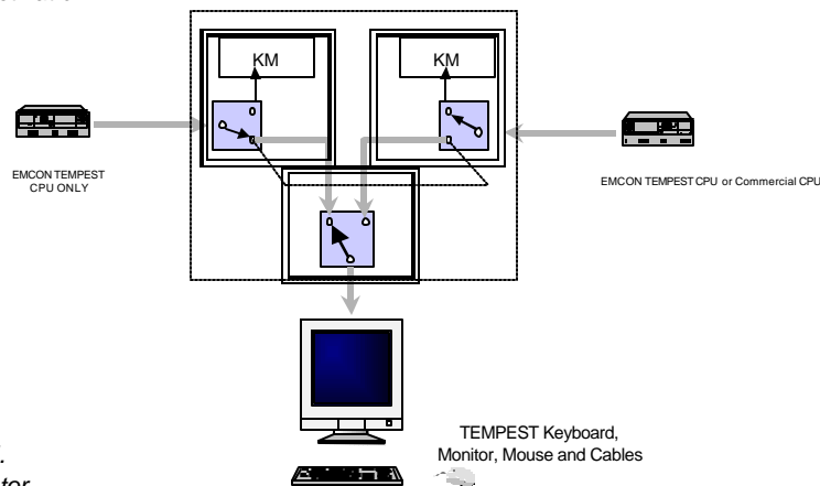
Diagram illustrates two-port model.
